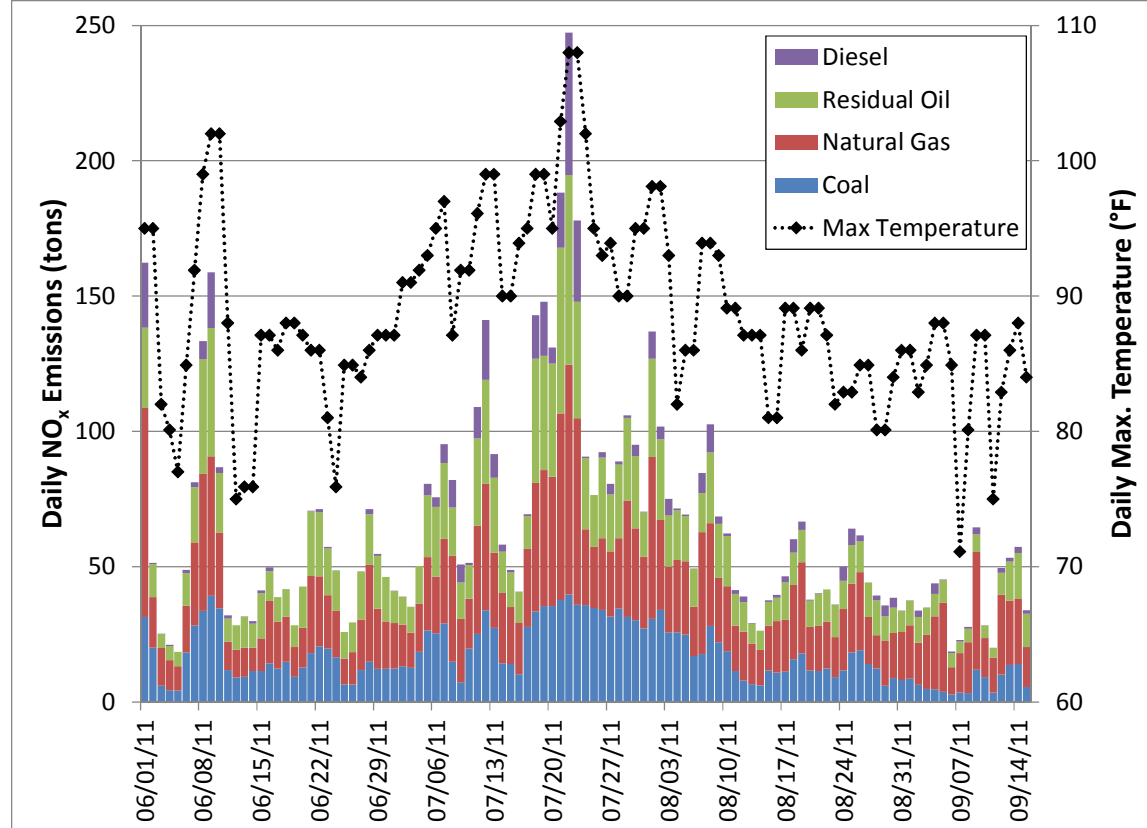
Figure 1. Daily NO x Emissions Variability from EGUs in NJ and Downstate NY Based on Fuel Type
